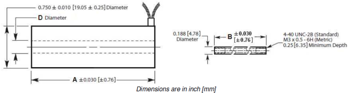
Figure 1: Mechanical specifications
